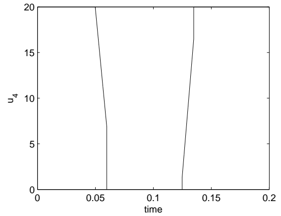
Figure 5.10: Control u_4 for problem 7
