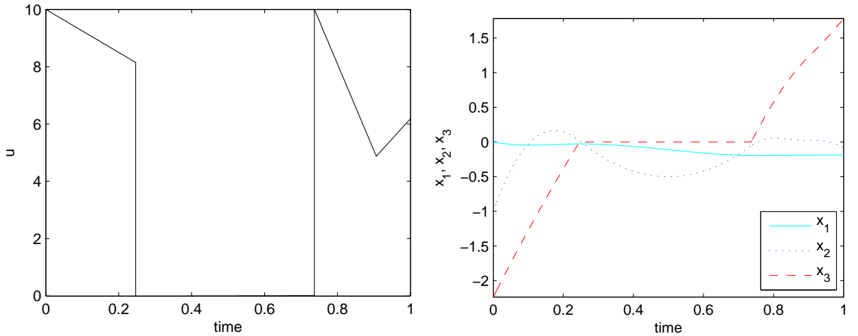
Figure 3.5: Control profile for unconstrained problem with gradients and bounds
